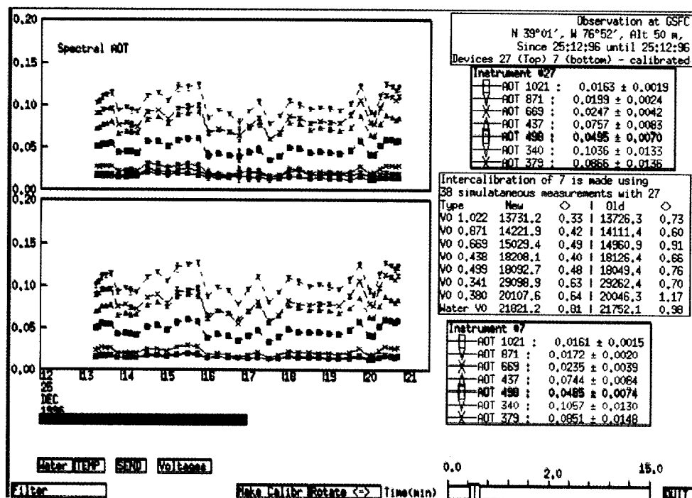
Figure 3. The intercomparison window which allows recomputation of V_0 values from a time series of AOTs of two simultaneously measuring instruments. AOTs from a reference instrument (top plot) are used with voltages from a field instrument (bottom plot) to compute a table of new V_0 's. Options to examine time-dependent voltage ratios may also be accessed from this window.
