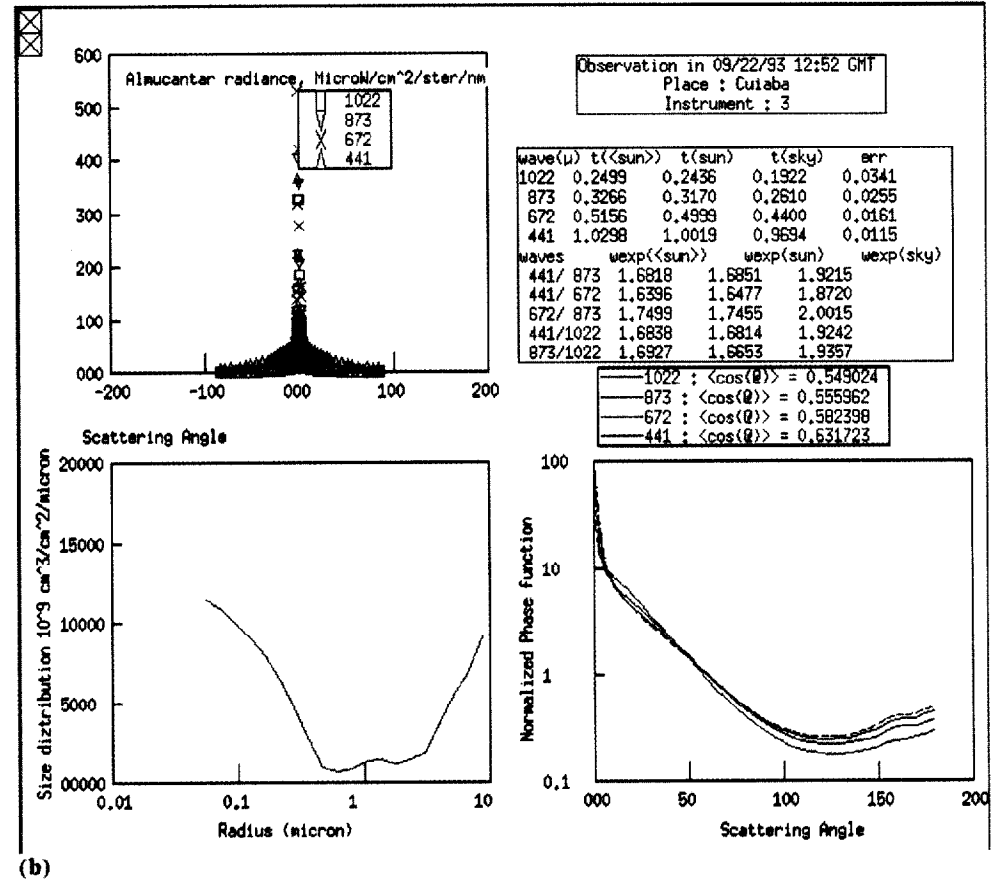
Figure 4b. A successful inversion of almucantar radiances during low aerosol loading is possible when the radiance data are symmetric about the Sun (upper left plot within window). Inversions produce a volume size distribution with good accuracy from 0.1 \mu\text{m} to about 8 \mu\text{m} aerosol radii (lower left window). The aerosol optical thickness and wavelength exponent are computed (upper right window) and compared to that measured by direct Sun observation. The spectral phase function and asymmetry factor (lower right side of window) from the aureole inversion are also computed using the "pak-rad" code of Nakajima et al. (1996).
