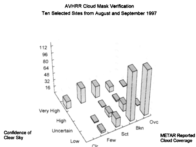
Figure 8. Comparison of surface cloud reports and AVHRR cloud mask results. Note the good agreement in clear as well as broken and overcast skies.
