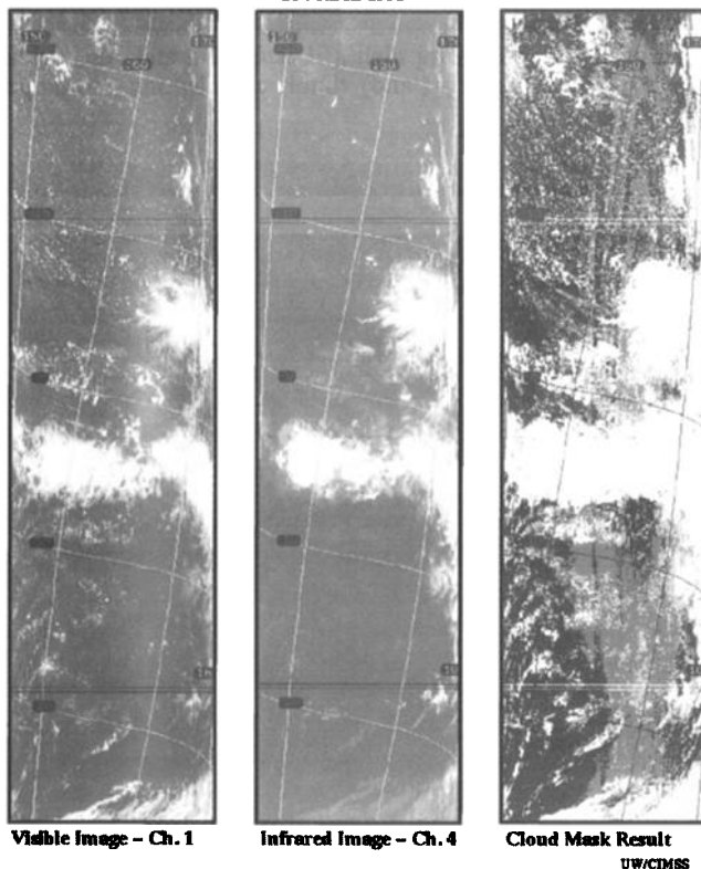
Figure 3. An example of the cloud mask derived from AVHRR data for a scene over the Pacific Ocean (right-hand panel), together with images from two of the AVHRR bands used in generating the mask. The legend is as follows: black is high confidence of clear (bits 1–2 equal 11), dark gray is probably clear (bits 1–2 equal 10), light gray is uncertain (bits 1–2 equal 01), and white is cloudy (bits 1–2 equal 00).
