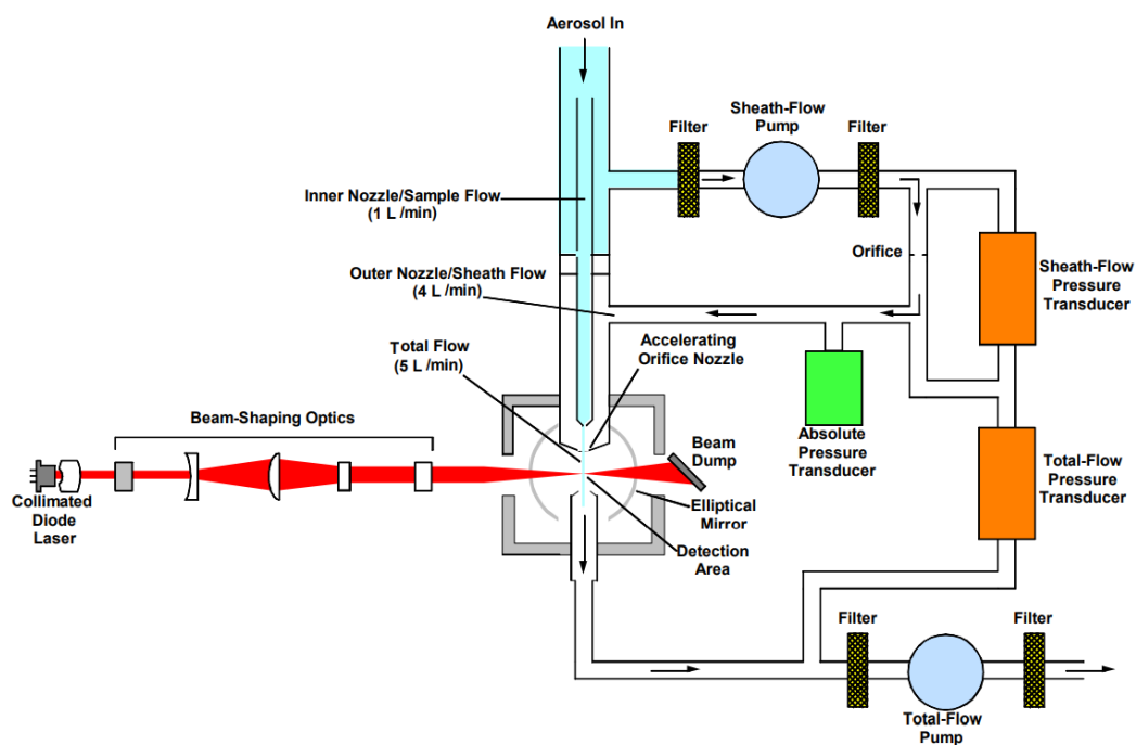
Figure 22: APS Instrument Theory of Operation
