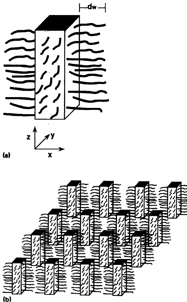
FIG. 1. (a) Single main pore with wall pores of length d_w . (b) Arrangement of main pores in the porous sample model. Wall pores are not taken to connect adjacent main pores. Air filled regions in (a) and (b) are dark.
