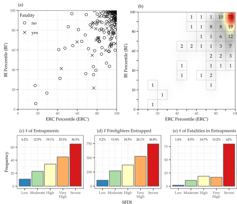
Figure 12. Associations between percentiles of the Energy Release Component (ERC'), the Burning Index (BI'), Severe Fire Danger Index (SFDI), and 178 wildland firefighter entrapments that occurred across CONUS between 1979 and 2017. (a) Scatterplot of fatal and non-fatal entrapments. (b) Density plot annotated with the number of entrapments per decile. (c), (d) and (e) The number of entrapments, the number of firefighters entrapped, and the number of firefighter entrapment fatalities that occurred in each class of SFDI. Note the floating y-axis on the bottom panels.
