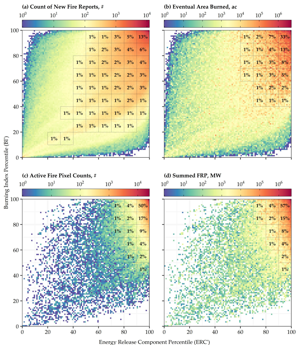
Figure 6. New and ongoing fire activity sorted into joint bins of the Energy Release Component (ERC') and Burning Index (BI') percentiles. At 1 percentile resolution the color scales indicate the amount of fire activity observed in each joint bin, and at decile resolution the percentages indicate the proportion of fire activity observed in each joint bin. Note the logarithmic color scales, and that percentages less than 1% are not labelled. (a) Counts of new fire reports contained in the FPA FOD. (b) Eventual area burned by new fires that started under those fire danger conditions. (c) Active fire pixel counts detected by MODIS. (d). Sum of FRP detected by MODIS.
