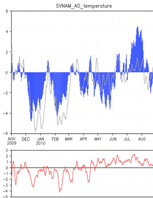
Fig. 1 (Top) Time series of the AO index (blue) as defined by Ogi et al. (2004), who called it the SV NAM index. For reference, the conventional AO index reported by NOAA/CPC is shown by the gray line. The vertical axis is dimensionless because the indices are normalized. Tick marks on the horizontal axis indicate the 1 day of each month. Updated daily time series from 1958 are available at http://www.bio.mie.u.ac.jp/kankyo/shizen/lab1/AOindex.htm . (Bottom) Time series of the temperature anomaly (K) at 925 hPa averaged northward of 32.5°N over the Eurasian continent. Anomalies are calculated according to the daily climatology of 32 years
