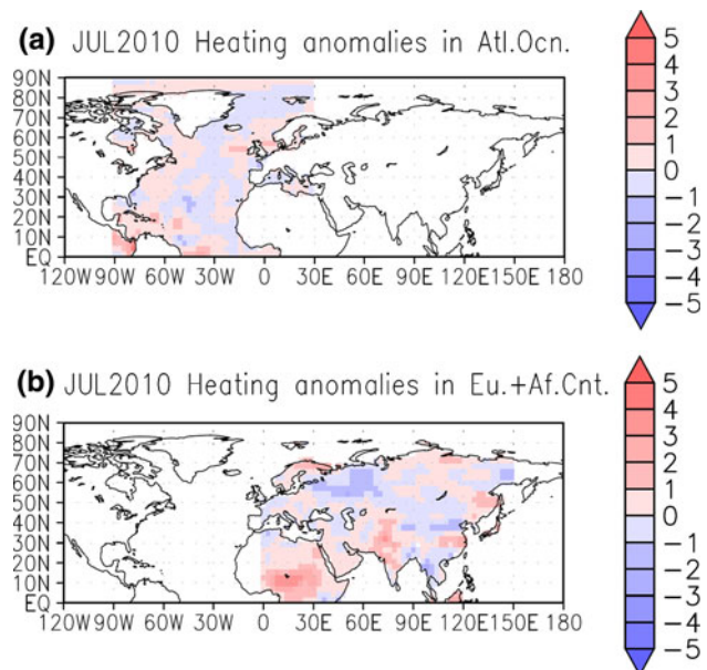
Fig. 6 Vertically averaged (from 0.7 to 0.3 \sigma ) diabatic heating derived from a conventional Q1 analysis (Yanai et al. 1973). The color scale indicates the heating anomaly ( \text{K day}^{-1} ) in July 2010 (deviation from the July climatological mean). a Heating anomalies over only the Atlantic Ocean (from 90°W to 30°E, from 0°N to 90°N). b Heating anomalies over only the Eurasian and African continent (from 0°E to 150°E, from 0°N to 90°N)
