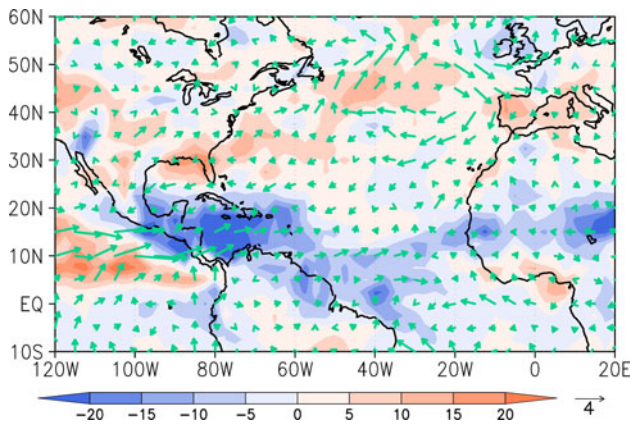
Fig. 5 OLR anomaly (color scale, \text{Wm}^{-2} ), defined as the deviation from the climatological temporal mean, on strongly positive AO days. Arrows show the surface wind anomaly ( \text{m s}^{-1} ) on strongly positive AO days, with the scale shown by the arrow below the lower right corner
