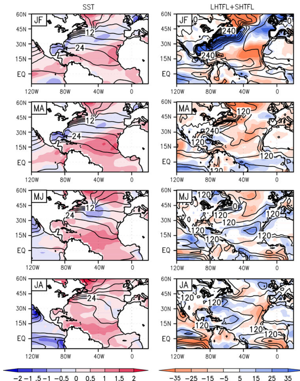
Fig. 3 Evolution of ( left column ) SST and its anomaly, and ( right column ) the sum of the latent and sensible heat fluxes and its anomaly, from January to August 2010. Contours show 2 month mean values, and the color shading shows the anomalies (deviations from the climatological temporal mean). JF, January and February;
