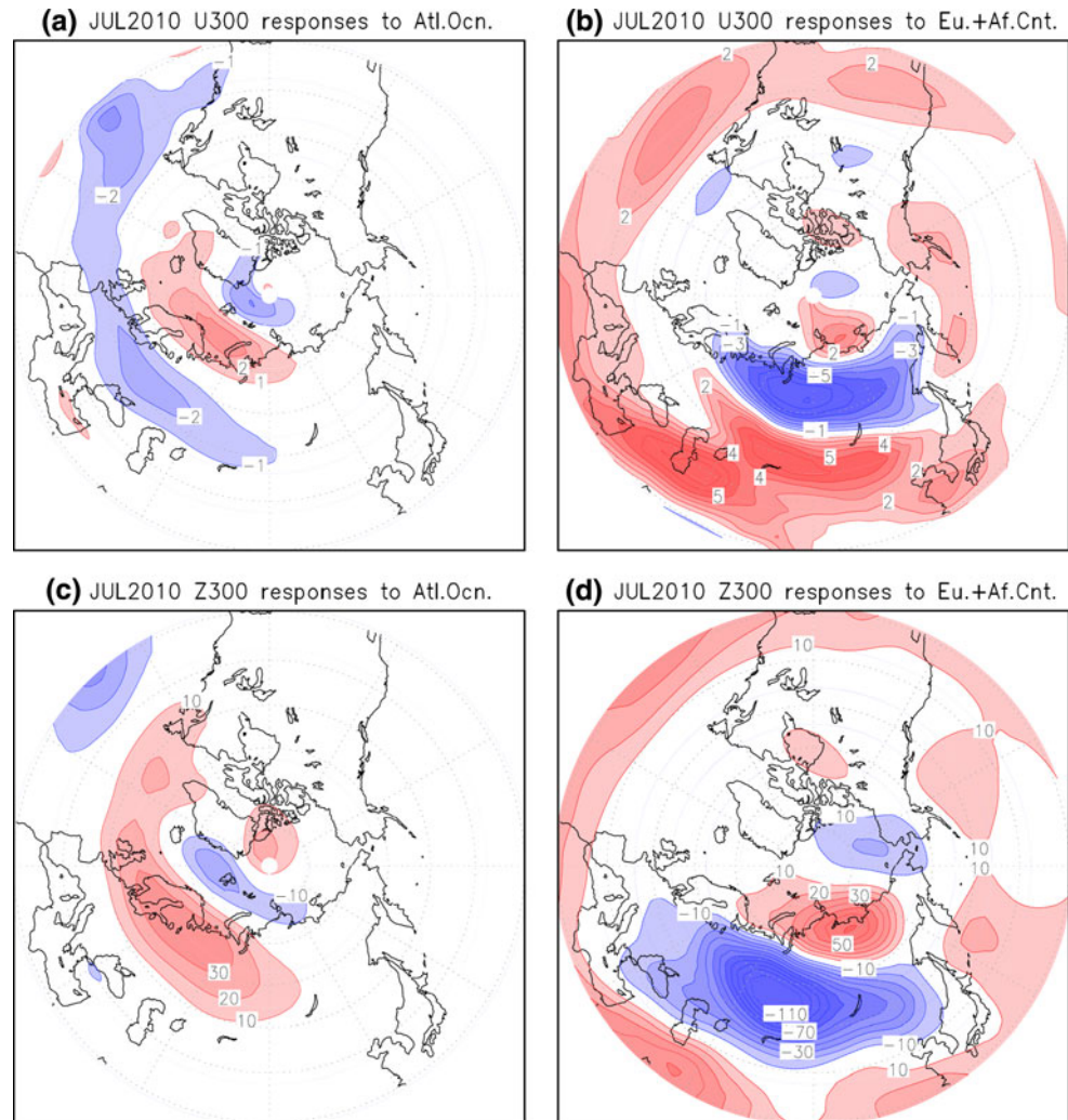
Fig. 7 a Steady responses of zonal wind at 300 hPa (U300) to the heating anomalies over the Atlantic Ocean, corresponding to those shown in Fig. 6a. Red/blue shading indicates positive/negative anomalies with units ( \text{m s}^{-1} ). b As in (a) except for responses to the heating anomalies over the Eurasian and African continent, corresponding to those shown in Fig. 6b. (c and d) As in (a) and (b) respectively except for geopotential height at 300 hPa (Z300) with units (m)
