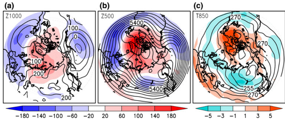
Fig. 4 Winter 2009/2010 (December, January, and February) mean geopotential height at 1000 hPa (a) and 500 hPa (b) and temperature at 850 hPa (c). Contours show winter mean values of geopotential height (contour interval 50 m) and temperature (contour interval 5 K). The color shading shows the geopotential height anomaly or the temperature anomaly from climatological temporal means
