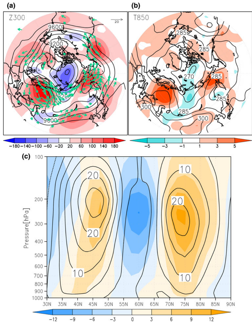
Fig. 2 a Time-mean geopotential height at 300 hPa, b temperature at 850 hPa (T850), and c vertical cross section of the eastward wind component at 135°E in the Northern Hemisphere during strongly positive AO days from 10 July to 4 August 2010. Contours show time-mean values of geopotential height ( a , contour interval 100 m), temperature ( b , contour interval 5 K), and wind speed ( c , contour interval 5 m s -1 ), and the color shading shows ( a ) the geopotential height anomaly, ( b ) the temperature anomaly, and ( c ) the zonal wind anomaly from climatological temporal means. The green arrows in ( a ) show the wave activity flux (m 2 s -2 ) at 300 hPa as formulated by Takaya and Nakamura (2001), with the scale shown by the arrow in the upper right corner
