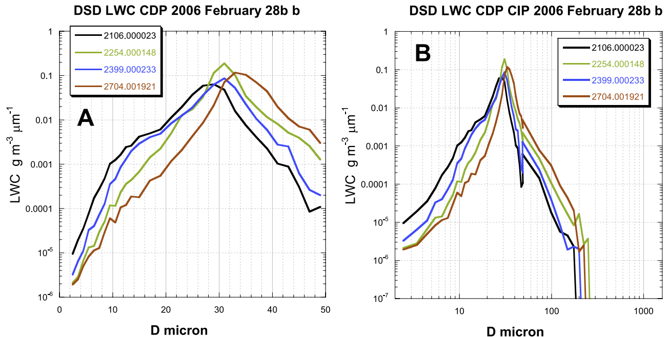
Figure 8. Same as Figure 7, but for Cloud 2 over the hills 60 km NE of Monterey (see location in Figure 6). It developed in an air mass that had 100 \text{ CCN cm}^{-3} . The cloud drops are quite large and the distribution continues smoothly into the raindrop sizes. This indicates active warm rain processes.
