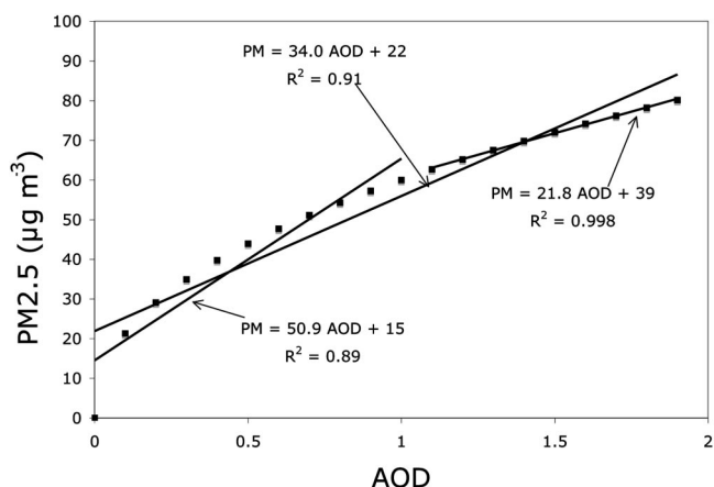
Figure 7. Hypothetical example of the slopes for low and high optical depths in which the model relationship follows Liu's 169 derived relationship (but scaled) PM_{2.5} = 60 \times AOD^{0.45} . Although the overall slope of the linear regression of all of the data is 34 μg · m -3 , it could be as high as 50.9 for the values <1 AOD and 21.8 for values from AOD of 1 to 2. The range of AOD observed would highly influence the slope and intercept in a linear model.
