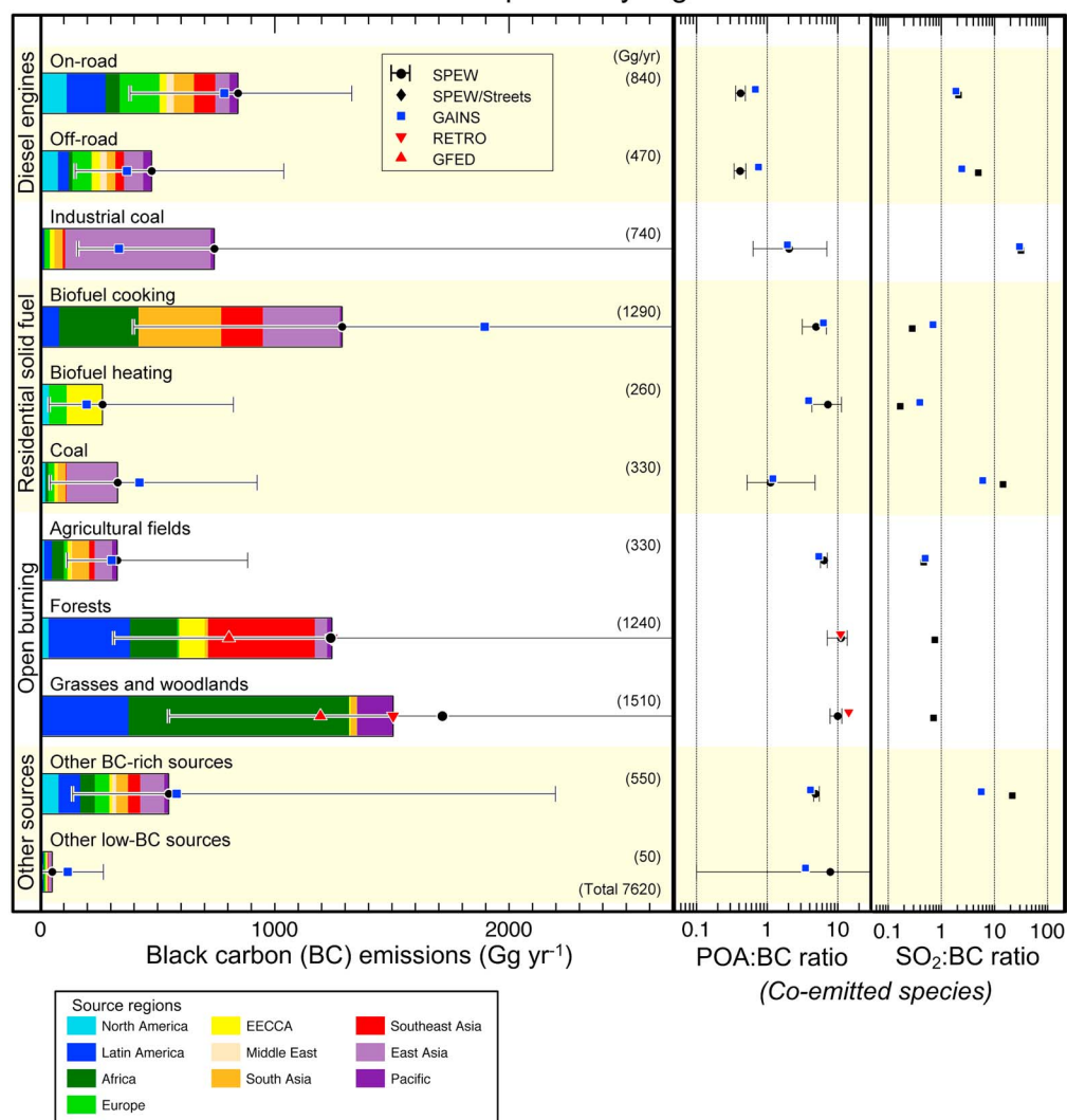
Figure 8. Emission rates of BC in the year 2000 by source category and ratios of co-emitted aerosols (e.g., primary organic aerosol, POA) and aerosol precursors (e.g., SO 2 ) to BC. For reference, it is often assumed that the ratio of OA to primary organic carbon (OC) varies from 1.1 to 1.4, depending on the source (section 3.2.2). SPEW emissions are shown as colored bars and are described by Lamarque et al. [2010]. GAINS estimates are from UNEP/WMO [2011a, 2011b], and RETRO emissions for open burning are described by Schultz et al. [2008]. Sulfur emissions from Streets et al. [2009] were used for ratios to SPEW. Regions are shown in Figure 7.
