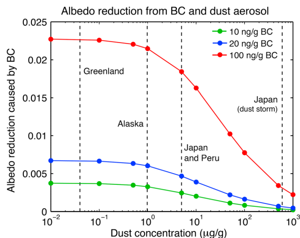
Figure 30. Reduction in hemispheric broadband snow albedo (0.3 to 5.0 \mu\text{m} ) caused by BC in the presence of varying amounts of dust. The perturbation caused by BC becomes smaller with increasing dust burden. Conditions represent a clear-sky atmosphere with solar zenith angle of 60^\circ and snowpack effective grain radius of 250 \mu\text{m} . Dust optical properties are similar to those listed in Flanner et al. [2009] for a particle effective radius of 1300 nm, and albedo calculations follow Flanner et al. [2009]. Vertical dashed lines depict, from left to right, dust-in-snow concentrations measured in Greenland ( 0.03\text{--}0.06\text{ }\mu\text{g g}^{-1} ) [ De Angelis et al. , 1997; Banta et al. , 2008]; Barrow, Alaska ( 0.98\text{ }\mu\text{g g}^{-1} ) [ Darby et al. , 1974]; Hokkaido, Japan, during pre-melt and Andes, Peru ( 5\text{ }\mu\text{g g}^{-1} ) [ Thompson et al. , 1979; Higuchi and Nagoshi , 1977]; and Hokkaido, Japan, after a dust storm ( 600\text{ }\mu\text{g g}^{-1} ) [ Aoki et al. , 2006].
