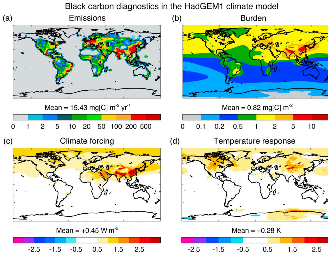
Figure 31. (a) Emissions of BC aerosols ( \text{mg BC m}^{-2} \text{ yr}^{-1} ), (b) burden of BC aerosols ( \text{mg BC m}^{-2} ), (c) direct radiative forcing due to BC aerosols ( \text{W m}^{-2} ), and (d) equilibrium surface temperature change (K) in response to the BC direct radiative forcing. Adapted from data from the Hadley Centre climate model (HadGEM1) published in Jones et al. [2007]. The patterns of burden, radiative forcing, and surface temperature response are considered illustrative because the lifetime of BC is known to be too long in this model.
