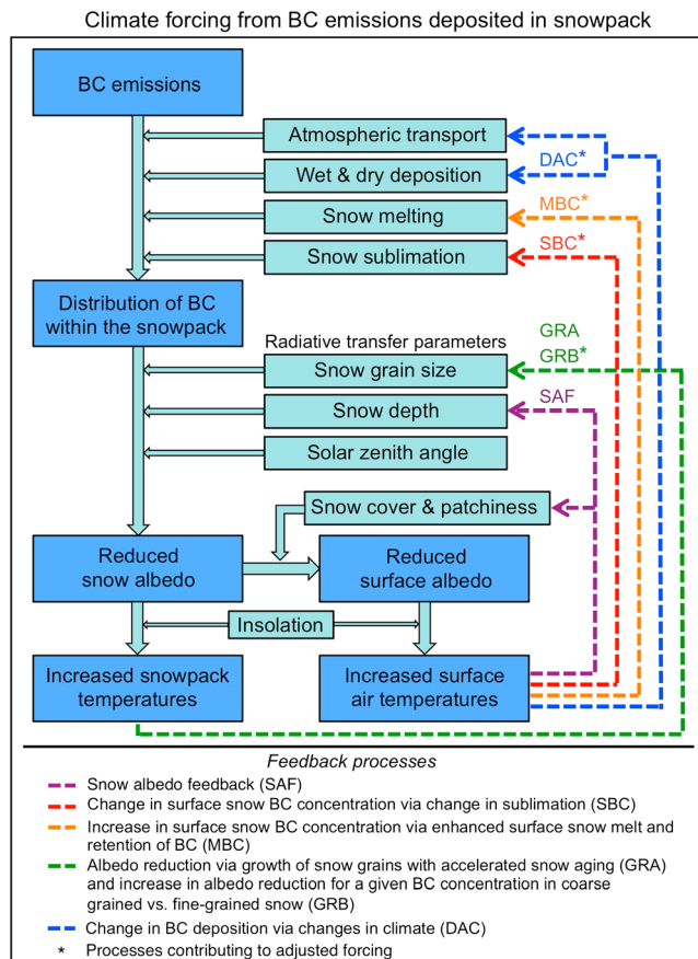
Figure 29. Schematic of the parameters and feedbacks that influence climate forcing by BC in surface snow. BC in the snowpack leads to reduced albedo of the snow surface, with the albedo change depending on BC amounts, snow grain size, and snow depth. Reduced snowpack albedo reduces regional surface albedo and leads to increased snowpack and surface air temperatures. The temperature changes feed back to snow albedo through changes in snow parameters via several processes, as noted in the legend and discussed in the text. This figure emphasizes feedbacks specific to forcing by BC in snow. Changes in climate of any origin may also affect BC emissions, atmospheric transport, rates of BC deposition to the snowpack, and snow accumulation rate.
