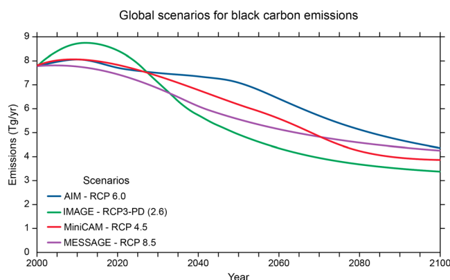
Figure 43. Total global BC emission projections from 2000 to 2100 in the four Representative Concentration Pathway (RCP) scenarios [Moss et al., 2010]. These scenarios are named according to the radiative forcing in 2100 and were developed by four individual modeling groups for use in climate modeling analysis for the IPCC Fifth Assessment Report. Decreasing emissions are a result of expectations of cleaner fuels use and declining emission factors with increasing income.
