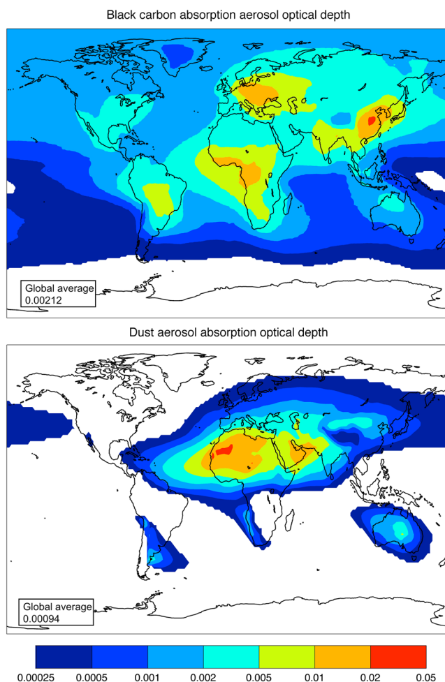
Figure 12. Aerosol absorption optical depth (AAOD) at 550 nm attributable to BC and dust. BC-AAOD fields are from the AeroCom median model fields [Schulz et al. , 2006] of all-source BC, including AAOD that would have been present before the pre-industrial era. Dust distribution is from Luo et al. [2003], with AAOD calculated from particle size in Mahowald et al. [2006] and optical properties in Yoshioka et al. [2007].
