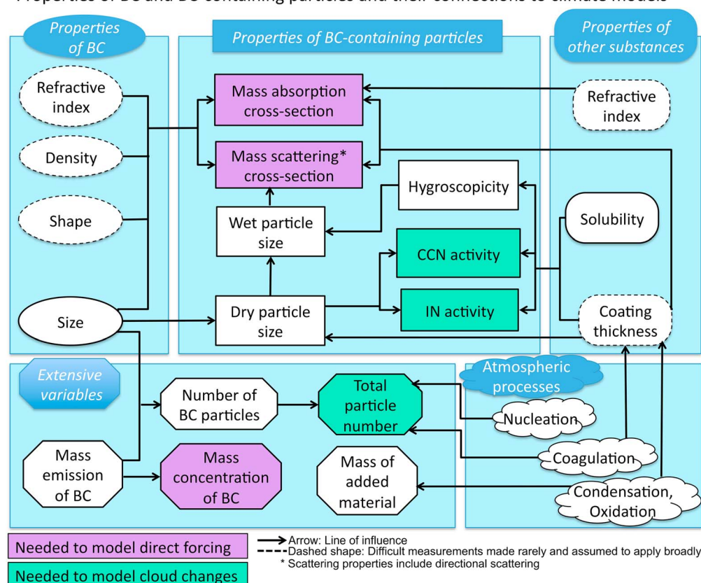
Figure 3. Schematic of the connections between properties of BC and BC-containing particles. A combination of these properties determines the contribution of BC and BC-containing particles to climate forcing. The properties depend on those of other substances produced in the atmosphere or co-emitted with BC and on atmospheric processes such as nucleation and condensation. Mass and number of BC and BC-containing particles (extensive variables) depend, in part, on particle properties that affect the lifecycle of BC (not represented here).
