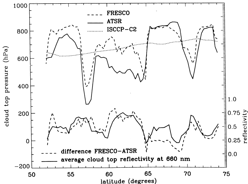
Figure 8. Cloud top pressures of FRESKO and ATSR-2, as well as their difference, in hPa. For comparison, the monthly average cloud top pressures from the ISCCP climatology are shown as well. The vertical axis on the right hand side pertains to the average cloud top reflectivity. The FRESKO and ATSR-2 data are from ERS-2 orbit 1337.
