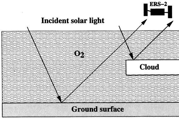
Figure 2. The two types of photon paths used in the FRESKO retrieval algorithm to simulate the spectrum of a partly cloudy pixel.
