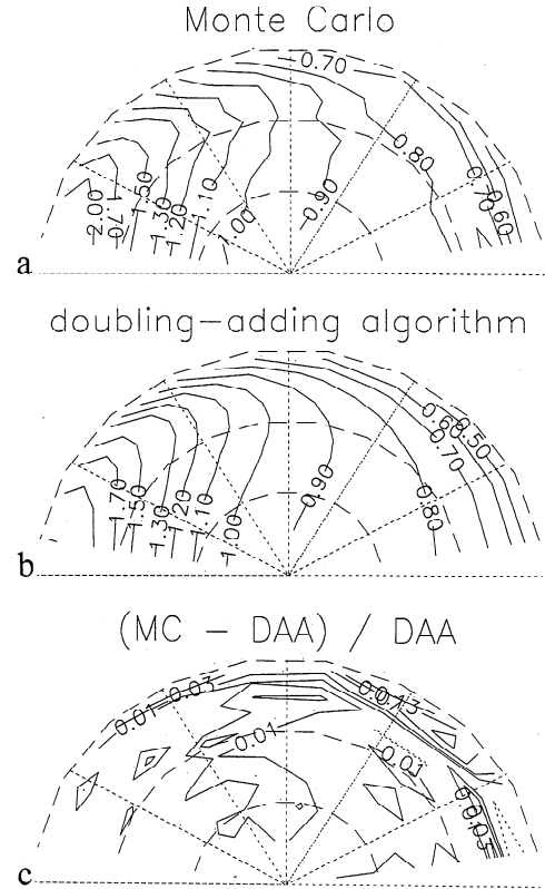
Figure 3. BRDF for overcast conditions obtained with (a) the Monte Carlo simulation for \tau = 50 and \theta_0 = 60^\circ and with (b) the doubling-adding algorithm (DAA) for the same parameters as with the Monte Carlo (MC) simulation. The radius of Figures 3a and 3b is a linear function of the viewing zenith angle \theta (with 0^\circ \leq \theta < 90^\circ ) and the polar angle is the viewing azimuth angle \phi (Sun is at 0^\circ , on the right-hand side) in increments of 30^\circ . The contour intervals are 0.1 between 0.0 and 1.3, and the other contour levels are 1.5, 1.7, 2.0, 2.5, and 3.0. (c) The discrepancies between the BRDFs. The contour levels in Figure 3c are equal to the relative error which is described by the ratio (MC-DAA)/DAA. The radius and the polar angle are the same as in Figures 3a and 3b. The contour levels are -0.05 (dotted line), 0.01, 0.03, 0.07, and 0.13.
