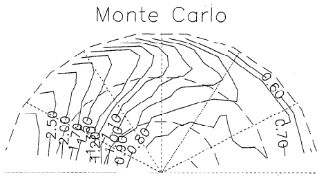
Figure 4. Same as Figure 3a, but for \tau = 6 .
