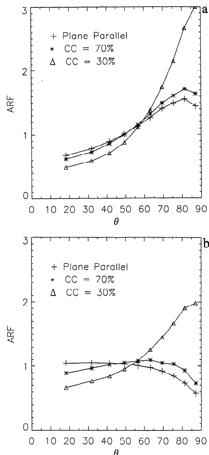
Figure 7. The ARF at various degrees of cloudiness obtained from the Monte Carlo model for (a) \tau = 6 and \theta_0 = 60^\circ and for (b) \tau = 20 and \theta_0 = 0^\circ .
