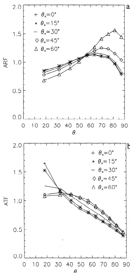
Figure 6. Same as Figure 5, but for \tau = 6 .
