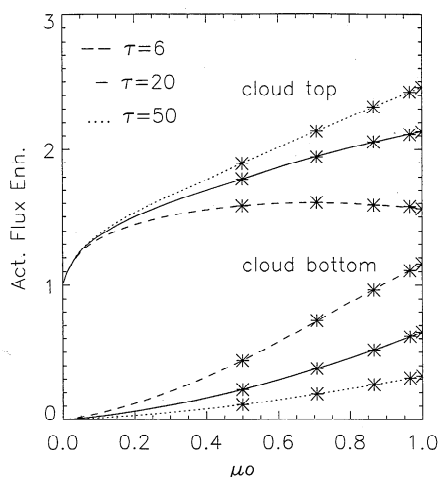
Figure 8. Actinic flux enhancement at cloud top and cloud bottom versus cosine of solar zenith angle, \mu_0 = \cos(\theta_0) , obtained with the doubling-adding algorithm for \tau = 6, 20 , and 50 . The asterisks indicate the results of the Monte Carlo simulation for the same conditions but for solar zenith angle \theta_0 between 0^\circ and 60^\circ in increments of 15^\circ .
