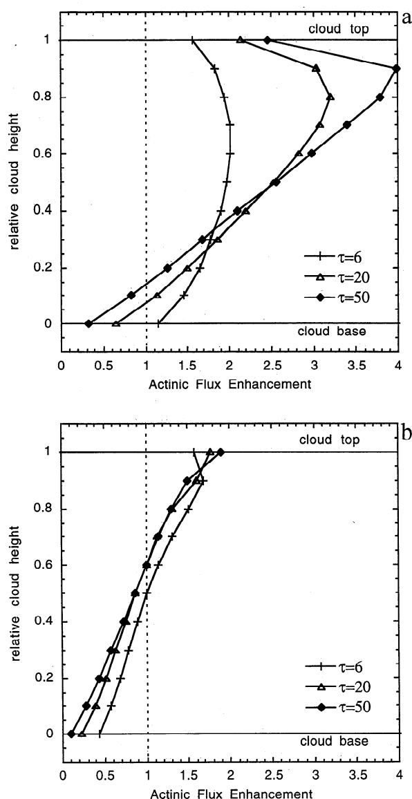
Figure 9. Actinic flux enhancement profiles in overcast conditions obtained with the Monte Carlo simulation for \tau = 6, 20 , and 50 and (a) \theta_0 = 0^\circ and (b) \theta_0 = 60^\circ . The horizontal lines at relative cloud heights I = 1.0 and 0.0 show the cloud top and cloud bottom, respectively. The dotted line indicates the actinic flux profile if no cloud is present.
