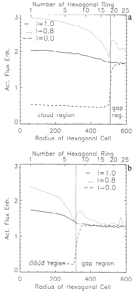
Figure 11. Horizontal actinic flux profiles from cloud center (hexagonal cell number 1) to the edge of hexagonal cell (hexagonal cell number 25) at relative cloud heights I = 1.0 (cloud top), 0.8 , and 0.0 (cloud bottom) obtained with the Monte Carlo model for \tau = 20 and \theta_0 = 0^\circ . Cloud cover c = (a) 70\% and (b) 30\% . The vertical line limits the inner cloud region.
