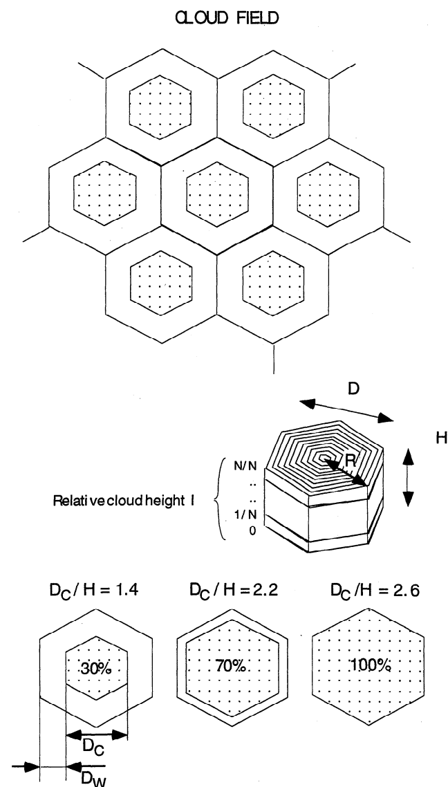
Figure 1. Geometry of the cloud field. A hexagonal cell consists of a core region (cloud cell) of hexagonal shape with “diameter” D_C and a wall region (cloud gap) of width D_W . The hexagonal cell is subdivided in 275 parts consisting of N = 11 vertically equidistant in-cloud surfaces (referred to as relative cloud heights) and 25 horizontally concentric hexagonal rings of equal area. The aspect ratio is equal to D_C/H , where H is the cloud height. The cloud cover c is 30%, 70%, and 100%. Cloud top and cloud base are flat surfaces. We use periodic boundary conditions; that is, the cloud field is stretched over a horizontally infinite domain.
