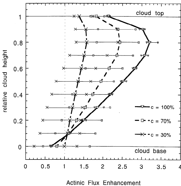
Figure 10. Vertical actinic flux profiles obtained with the Monte Carlo model for \tau = 20 and \theta_0 = 0^\circ at various degrees of cloudiness. The maxima and minima are given for each relative cloud height. The horizontal lines at relative cloud heights I = 1.0 and 0.0 show the cloud top and cloud bottom, respectively. The dotted line indicates the actinic flux profile if no cloud is present.
