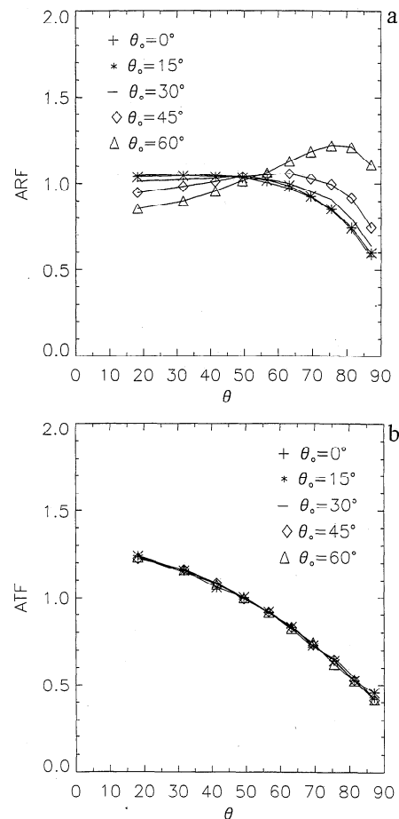
Figure 5. The (a) azimuth-averaged reflectance distribution function (ARF) and (b) the corresponding azimuth-averaged transmittance function (ATF) versus viewing zenith angle \theta obtained with the Monte Carlo model for \tau = 20 at various solar zenith angles \theta_0 .
