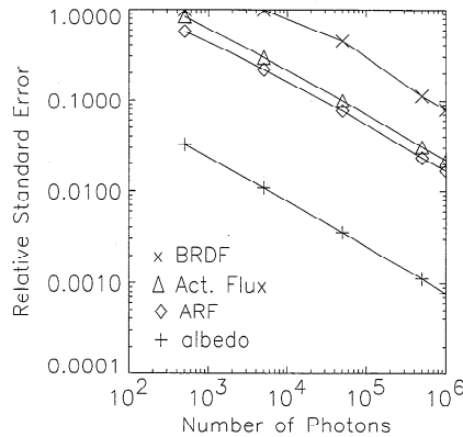
Figure 2. Log-log plot of the relative standard error of the albedo, the azimuth-averaged reflectance distribution function (ARF), the actinic flux enhancement, and the bidirectional reflectance distribution function (BRDF) versus the number of photons used in the Monte Carlo simulation. The curves show that the simulations are proportional to the binomial 1/\sqrt{N} law. The simulations are obtained for \tau = 20 and \theta_0 = 0^\circ .
