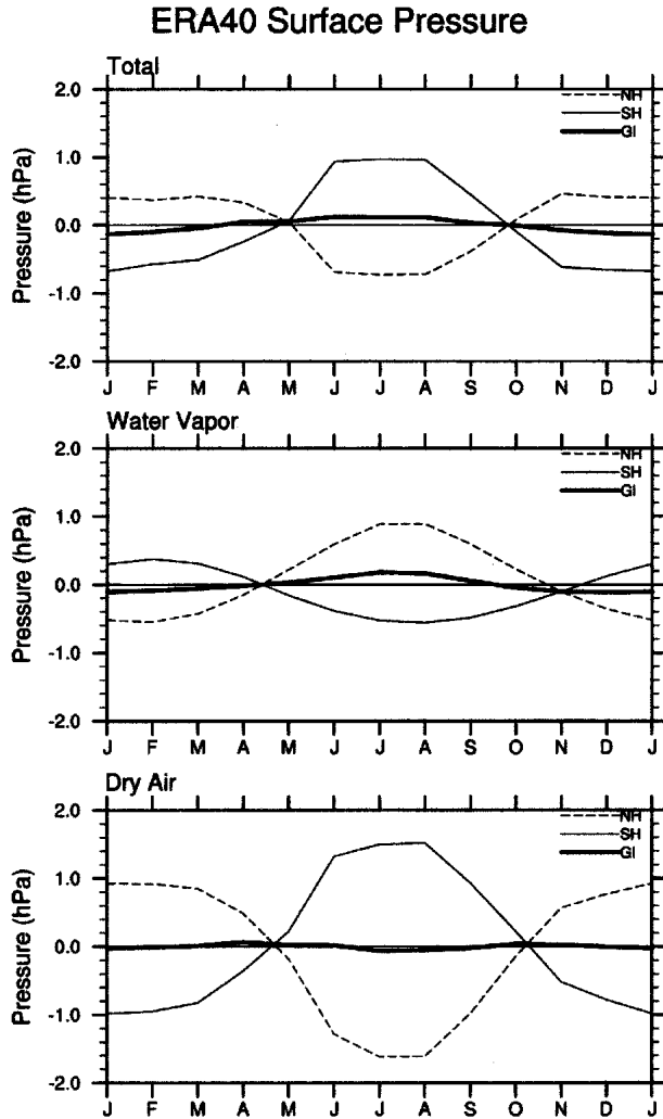
FIG. 3. Mean annual cycle of the hemispheric and global mean surface pressure anomalies relative to 1979–2001 means for (top) the total p_s , and contributions from (middle) water vapor p_w and (bottom) dry air p_d for ERA-40. The units are in hPa.
