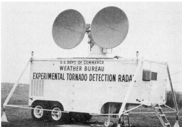
FIG. 2. USWB's continuous-wave 3-cm Doppler radar with its side-by-side transmitting and receiving antennas used for tornado studies in the southern plains during the late 1950s. The unit was converted by NSSL into a pulsed Doppler radar in 1964. [USWB photo.]
