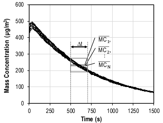
Figure 3: Extraction of the time-averaged mass concentration values ( \overline{MC}_i ) for several Sensirion PM sensors. In order to evaluate precision, sensors are individually averaged over the same time period \Delta t and \overline{MC}_i values are collected in a distribution.
