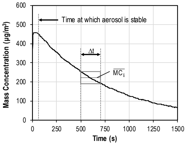
Figure 2: Extraction of the time-averaged mass concentration value ( \overline{MC}_i ) for a Sensirion PM sensor. In order to filter out the impact of the statistical noise of the measurement, concentration is averaged over a time period \Delta t .
