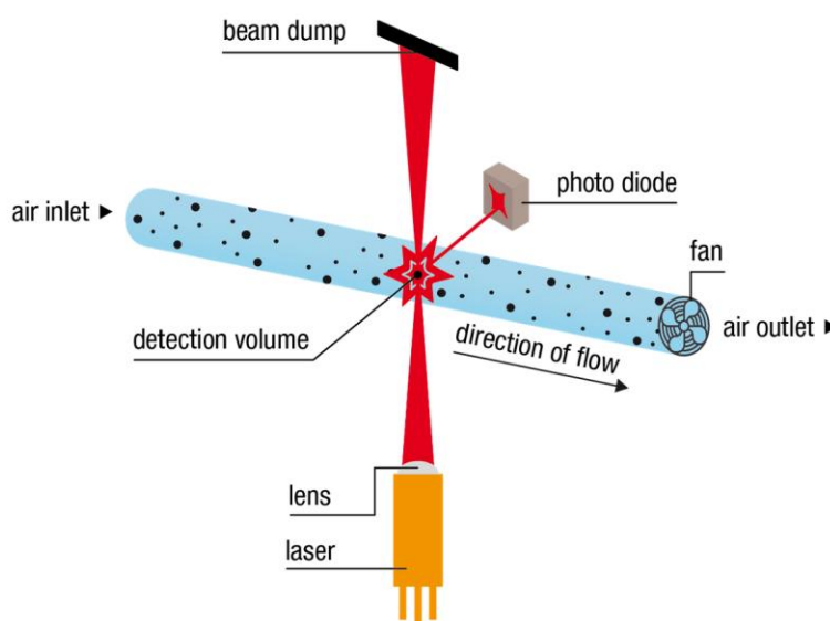
Figure 1 Measurement principle of Sensirion PM sensors.
