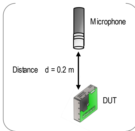
Figure 6: Measurement setup for the acoustic emission level test.
