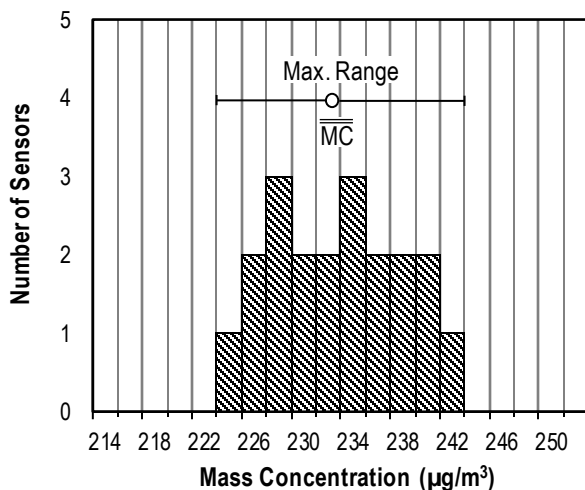
Figure 4: Extracted distribution of sensor deviation around average. Max. range must fit into specification band (see also Figure 5). \overline{MC} denotes the sensor sample average.
