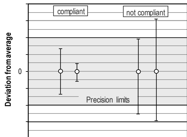
Figure 5: Examples for sensor distributions complying (left side) or not complying (right side) with the specified precision range. Open dots represent average values. Error bars denote max. range and must stay within precision limits.
