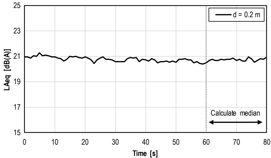
Figure 7: Measurement data for acoustic emission level in dB(A) for the typical SPSxx PM sensor at a distance of 0.2 meters.
