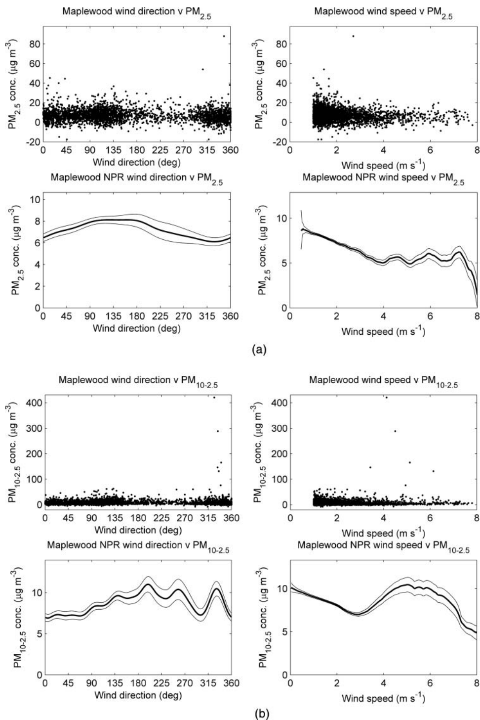
FIG. 5. NPR results for (a) \text{PM}_{2.5} ( n = 2930 ) and (b) \text{PM}_{10-2.5} ( n = 2930 ) mass concentrations ( \mu\text{g m}^{-3} ) at Maplewood, showing relationships with wind direction (degrees clockwise from north) and wind speed ( \text{m s}^{-1} ).
