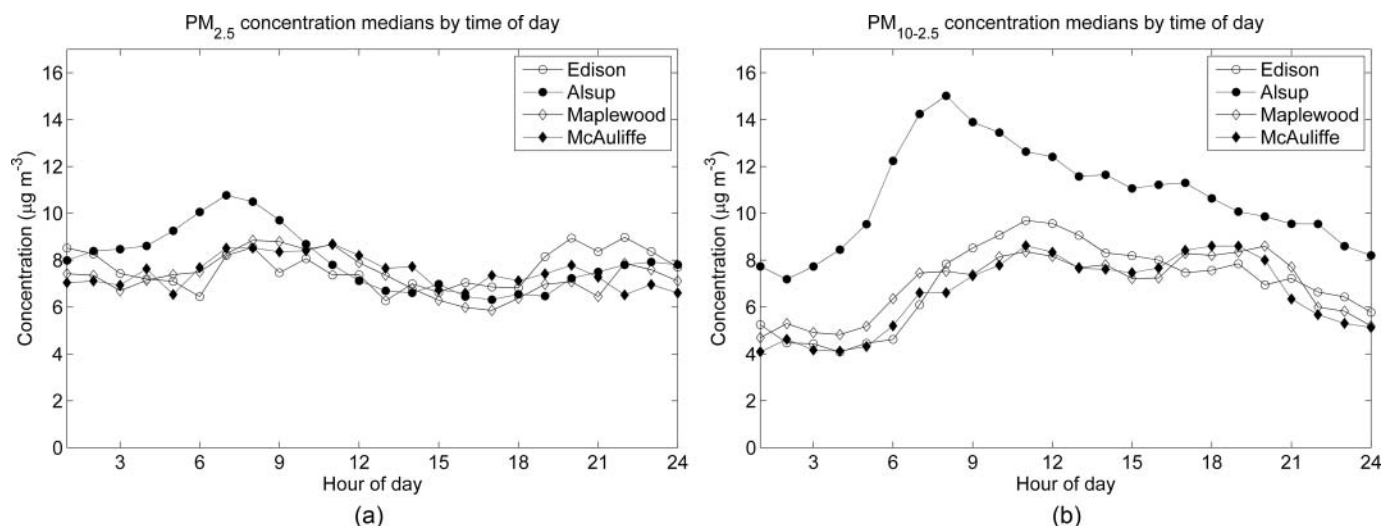
FIG. 1. Median mass concentrations ( \mu\text{g m}^{-3} ) by time of day at the 4 monitoring sites for (a) \text{PM}_{2.5} and (b) \text{PM}_{10-2.5} .
