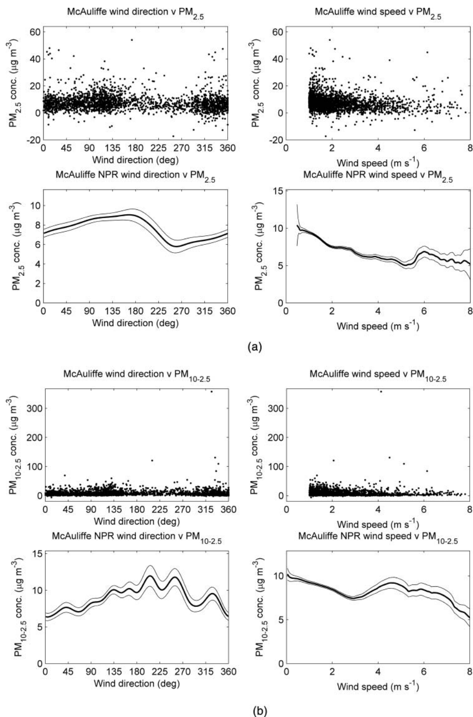
FIG. 6. NPR results for (a) PM_{2.5} ( n = 2262 ) and (b) PM_{10-2.5} ( n = 2262 ) mass concentrations ( \mu\text{g m}^{-3} ) at McAuliffe, showing relationships with wind direction (degrees clockwise from north) and wind speed ( \text{m s}^{-1} ).
