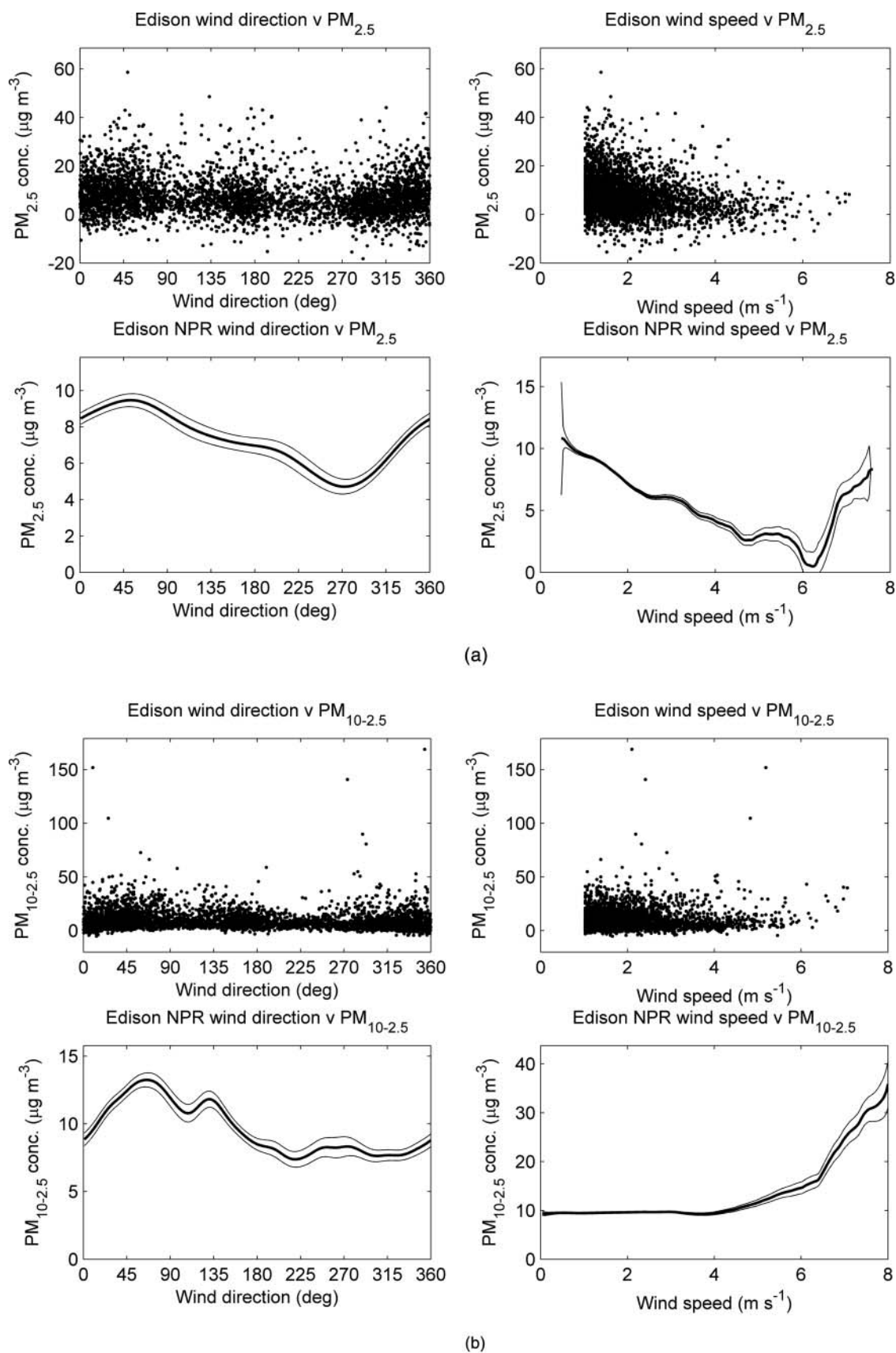
FIG. 3. NPR results for (a) PM_{2.5} ( n = 4028 ) and (b) PM_{10-2.5} ( n = 4028 ) mass concentrations ( \mu\text{g m}^{-3} ) at Edison, showing relationships with wind direction (degrees clockwise from north) and wind speed ( \text{m s}^{-1} ).
