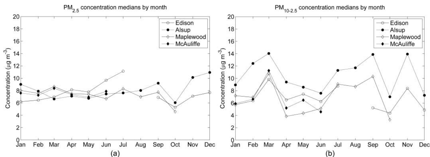
FIG. 2. Monthly median mass concentrations ( \mu\text{g m}^{-3} ) at the 4 monitoring sites for (a) \text{PM}_{2.5} and (b) \text{PM}_{10-2.5} .
