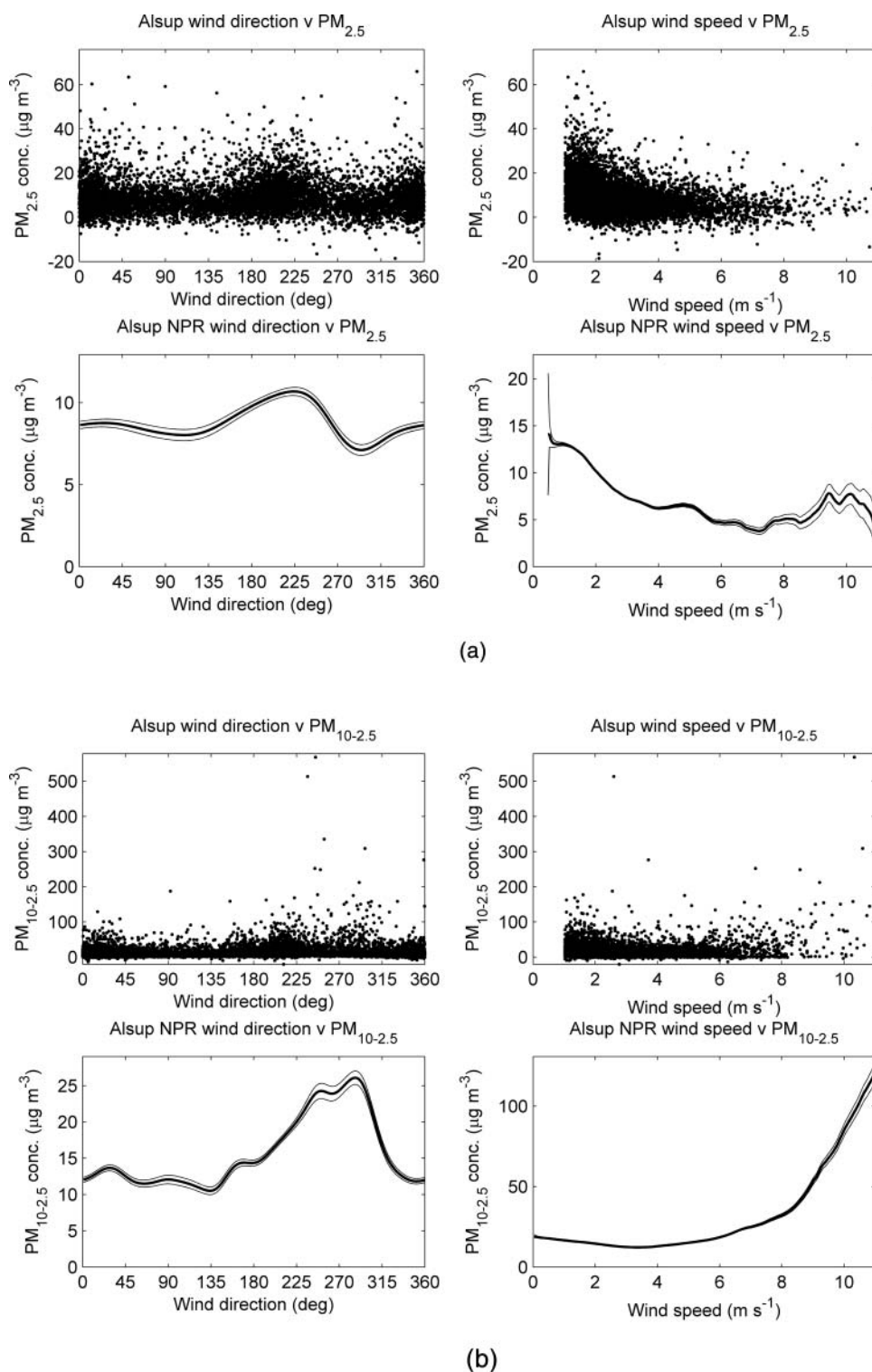
FIG. 4. NPR results for (a) PM_{2.5} ( n = 7626 ) and (b) PM_{10-2.5} ( n = 7496 ) mass concentrations ( \mu g m^{-3} ) at Alsup, showing relationships with wind direction (degrees clockwise from north) and wind speed ( ms^{-1} ).
