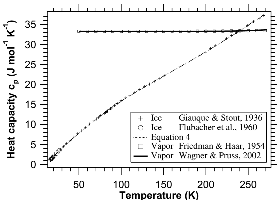
Figure 1. The molar heat capacities of ice and water vapour. The vapour-phase heat capacities from Wagner and Pruss (2002) include non-ideal-gas effects but those from Friedman and Haar (1954) do not.
