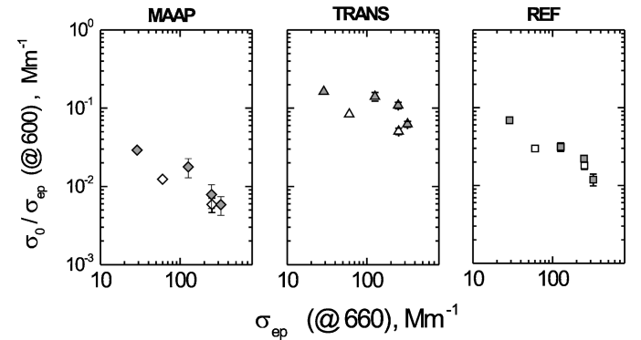
Figure 12. Method response to white aerosol displayed as ratio \sigma_0/\sigma_{\text{ep}} : open symbols, PSL spheres; filled symbols, ammonium sulphate.
