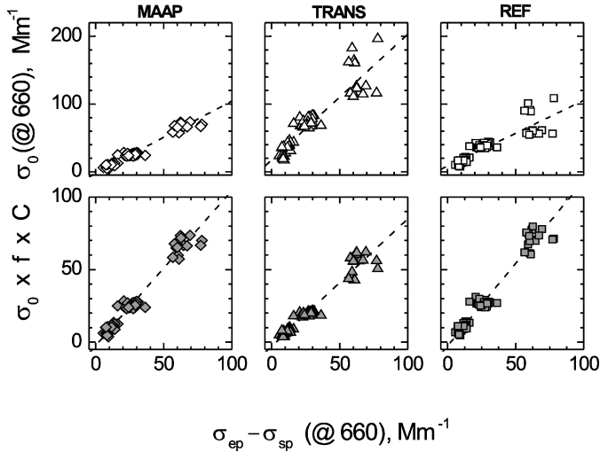
Figure 8. Method-dependent response coefficient \sigma_0 measured with MAAP, TRANS, and REF, respectively, as a function of the reference value \sigma_{ap} = \sigma_{ep} - \sigma_{sp} : externally mixed graphite soot–ammonium sulphate aerosol; dashed lines give the linear regression lines. Top row panels represent uncorrected data \sigma_0 , bottom row panels represent data corrected for filter-loading and aerosol-scattering effects \sigma_0 \times f \times C .
